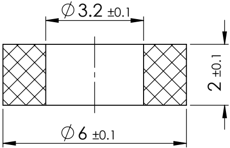
SECTION X-X
